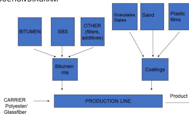
PRODUCTION DIAGRAM
